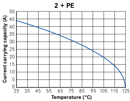
all contacts \varnothing 2,5 mm Pin 4mm 2 - Socket 6mm 2
