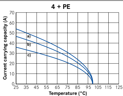
all contacts \varnothing 2,5 mm a) 4 contacts loaded 6mm 2 b) 4 contacts loaded 4mm 2 c) 4 contacts loaded 2,5mm 2
