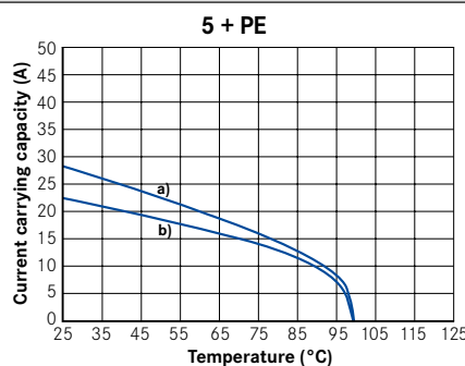
all contacts \varnothing 2,5 mm a) wire gauge 4,0 mm 2 b) wire gauge 2,5 mm 2
