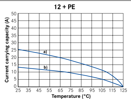
a) 4 contacts \varnothing 2,5 mm, wire gauge 2,5 mm 2 b) 9 contacts \varnothing 1,6 mm, wire gauge 2,5 mm 2
