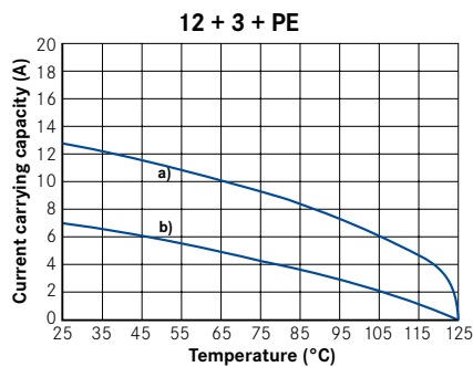
a) 4 contacts \varnothing 1,6 mm, wire gauge 1,5 mm 2 b) 12 contacts \varnothing 1,5mm, wire gauge 0,5 mm 2
