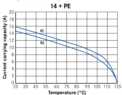
a) 11 contacts \varnothing 1,6 mm, wire gauge 1,5 mm 2 b) 4 contacts \varnothing 1,5mm, wire gauge 0,5 mm 2
